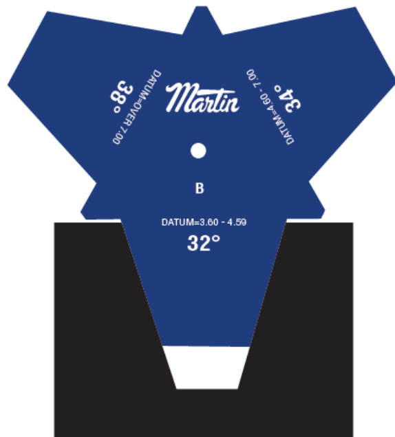
Normal Sheave (Uniform Angle)
