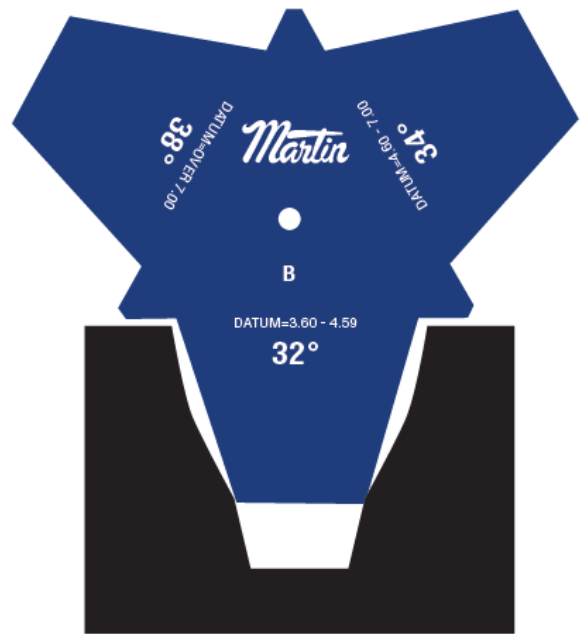
Worn Sheave (Dished Out)
